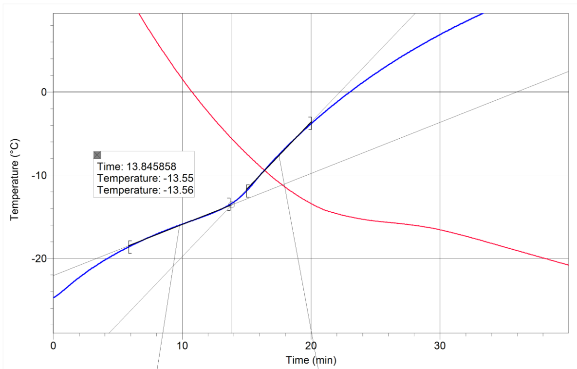
Thawing curve (blue) processing
