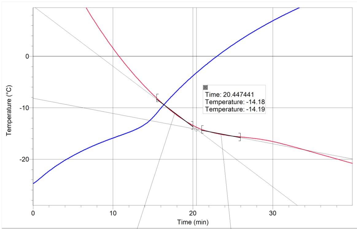
Freezing curve (red) processing
